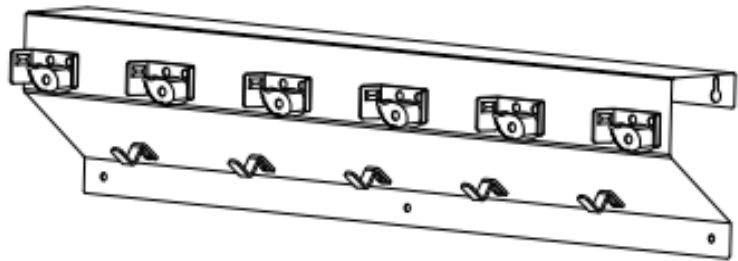
PERSPECTIVE
