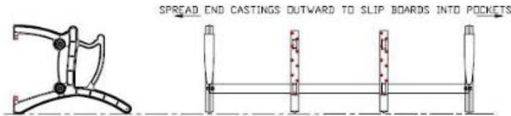
Diagram 2: Placing and Fastening "Seat" Boards In Place
