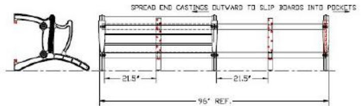
Diagram 4: Placing & Fastening Back Boards in Both Sections - One Section At A Time
