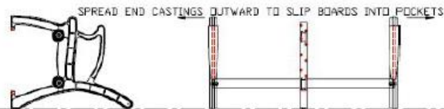
Diagram 1: End Casting and Support Tube Assembly
