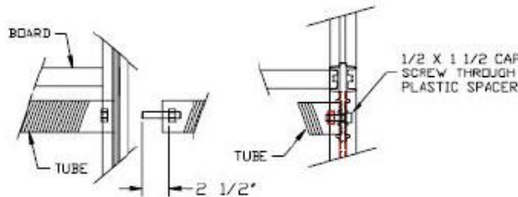
Detail A: Cap Screws & Threaded Rod Attachment
