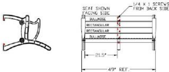
Diagram 2: Placing and Fastening Seat Boards - Section 1
