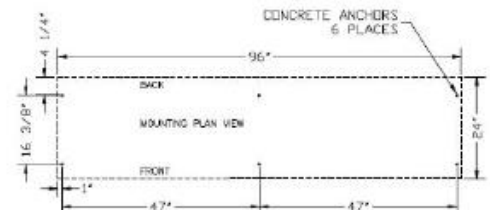
Diagram 5: Surface Mounting Instructions
