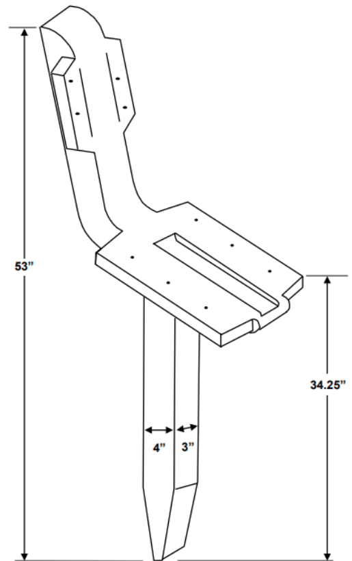
In-ground bench leg
