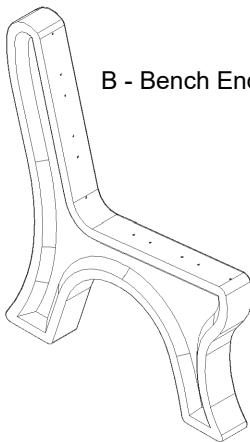
( 4 ) - Four Bench Ends PS-SBBE-H-03
