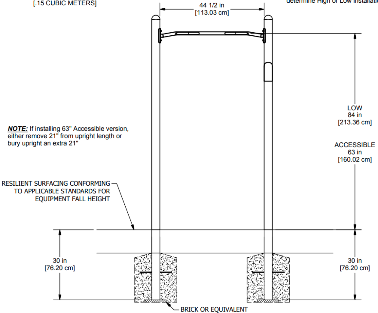
ELEVATION VIEW
