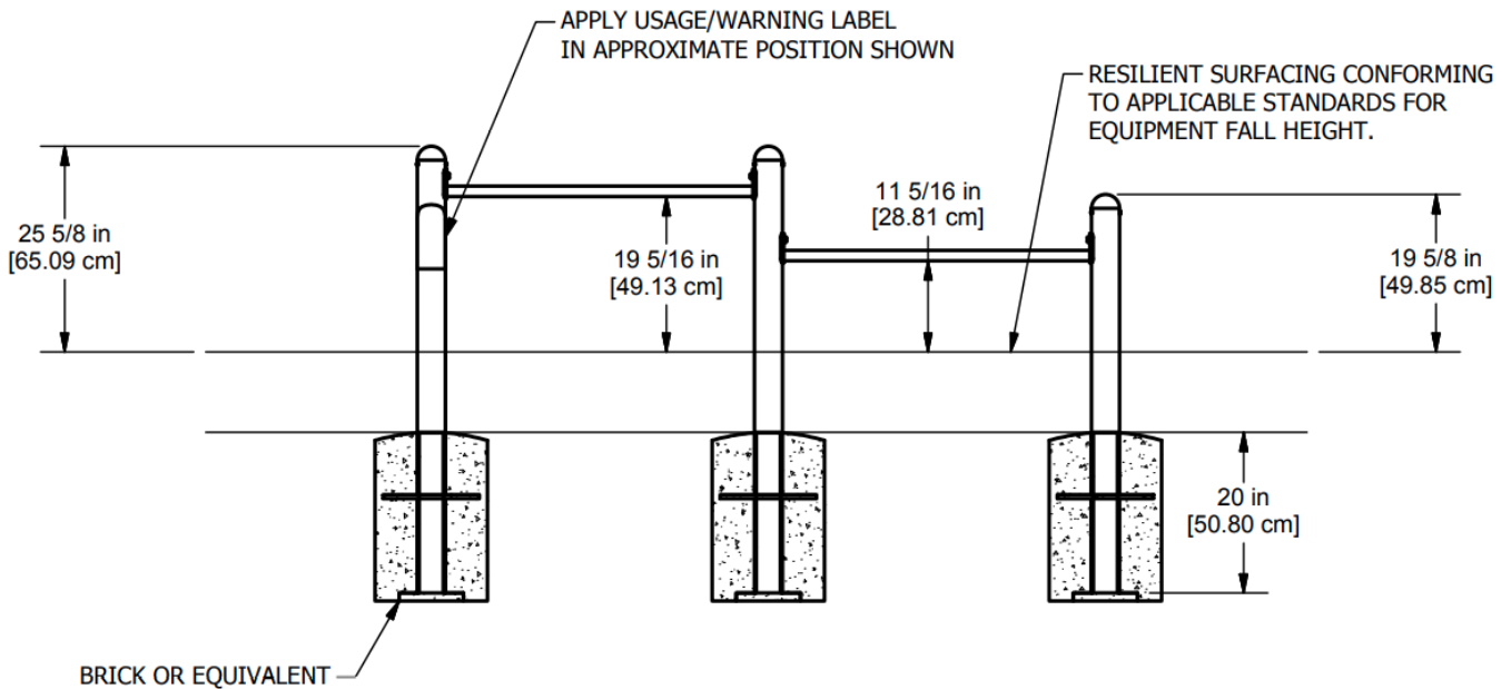
ELEVATION VIEW
