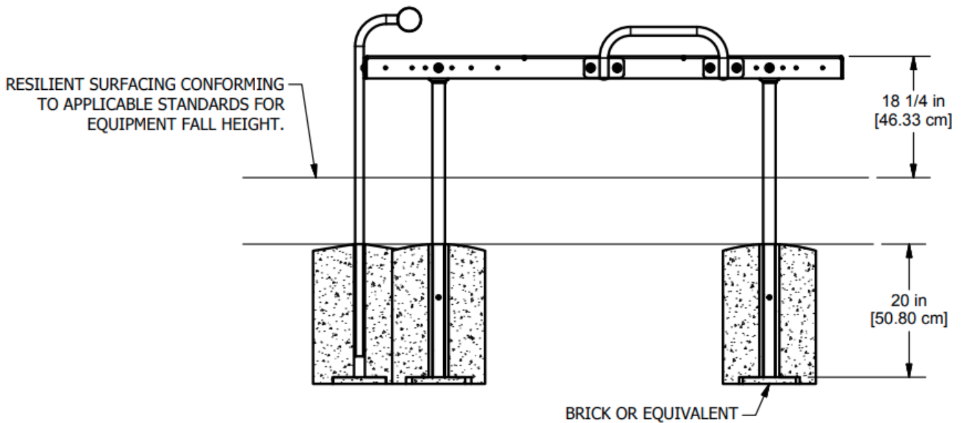
ELEVATION VIEW
