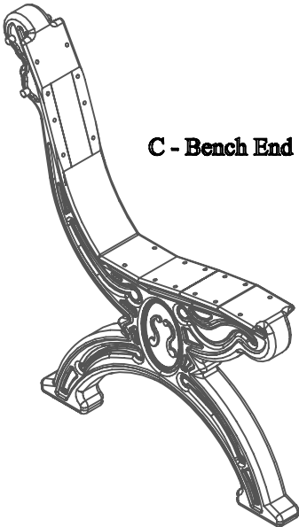
( 2 ) - Two Bench Ends PS-CBBE-A-01
